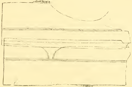
Fig. 2. Coscinodiscus subbuliens Jørg. An empty and partly broken frustule. Height 85 \mu . 506 t. m.
